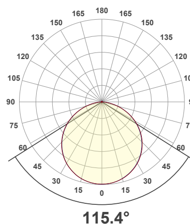
FF2-SW-10W-30K-IP20-24V-TB
