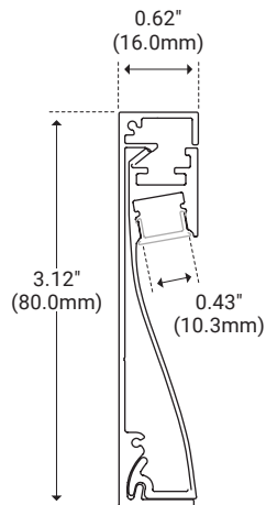
Aluminum Profile 1
