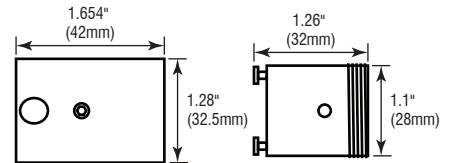
CM—Ceiling Mount
