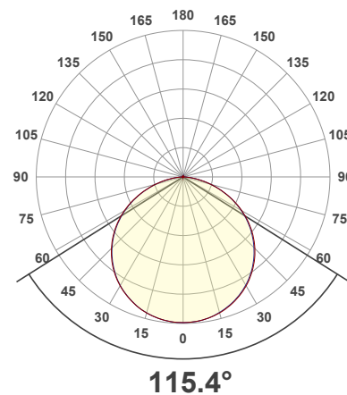
FF2-SW-10W-30K-IP20-24V-TB
