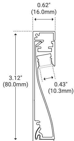
Aluminum Profile 1
